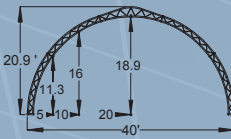
40' Freestanding
